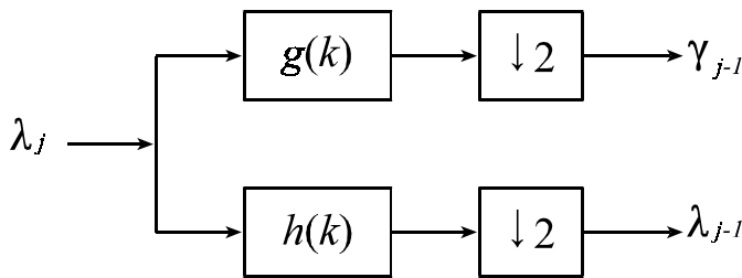
Figure 5 Implementation of equations (23) and (24) as one stage of an iterated filter bank.
